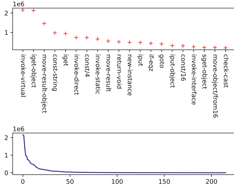
Figure 3.2. Opcode frequency across the pre-training corpus. The upper panel names the twenty most common operations, and the lower panel plots all 216 in rank order. The figure describes empirical frequencies, without a statistical test of a power-law fit. Reproduced from [5].
