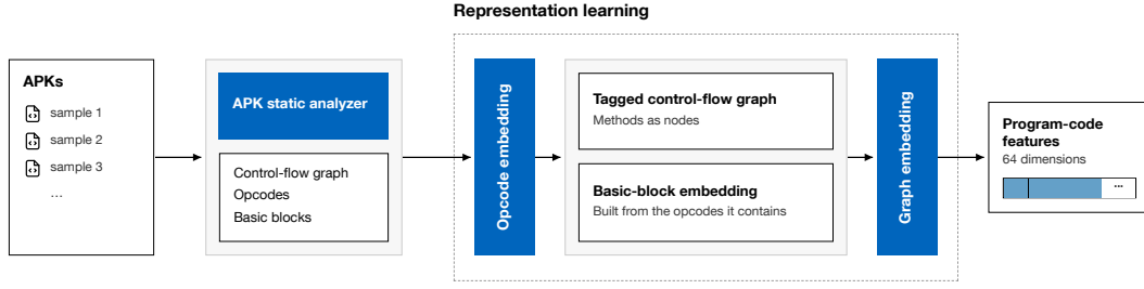
Figure 3.3. Published design of the program-code branch, redrawn by the candidate from [5].
