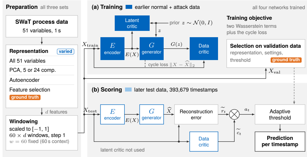
Figure 5.7. Multivariate GAN detection pipeline. (a) The four networks are trained together on earlier windows containing normal and attack observations; validation data select the representation, the settings and the threshold. (b) The later 393,679 test timestamps are scored with the trained networks; the latent critic has no part in the score a_t of Equation 5.1. The blue tag marks the input representation, the only factor varied between runs, and orange tags mark the steps that used attack ground truth. The window length is fixed at 60 samples. The scaler and PCA are fitted on training data and reused for validation and testing. The candidate implemented every processing step shown.
