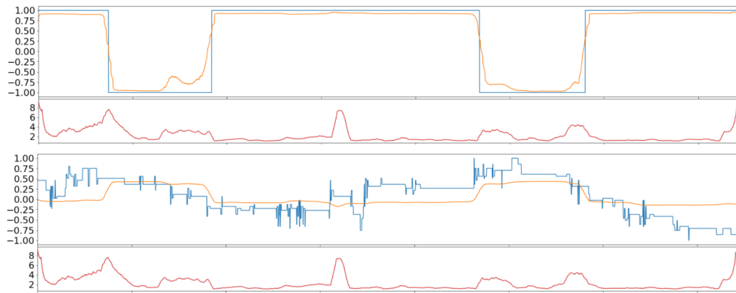
Figure 5.8. Observed signals (blue) and their reconstructions (orange) for two dimensions, reproduced at the original embedded resolution from Figure 4.15 of the internal report. The repeated red trace is the aggregate reconstruction discrepancy across dimensions, shared by the two displayed signals. It precedes the combination of Equation 5.1.
