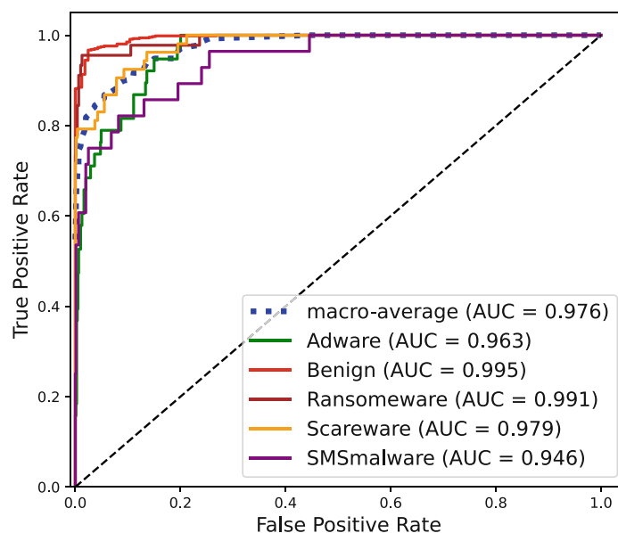
Figure 4.9 Per-class receiver operating characteristic curves for gradient boosting on the fused representation, reproduced from the published vector content of Figure 10 in [35]. The legend reports a macro-average AUC of 0.976 and the AUC of each class. The paper provides no selected operating threshold or fold-level variation.
