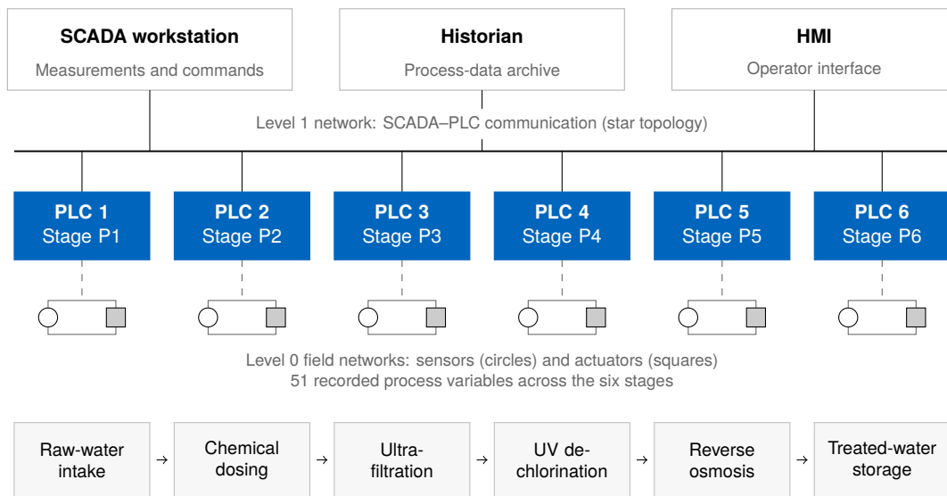
Figure 3.5 SWaT process and control architecture. Network levels follow the SWaT convention. The field-network symbols indicate sensors and actuators within each stage; the detector consumes their recorded values. Adapted from the supplied diagram and the dataset description [123].
