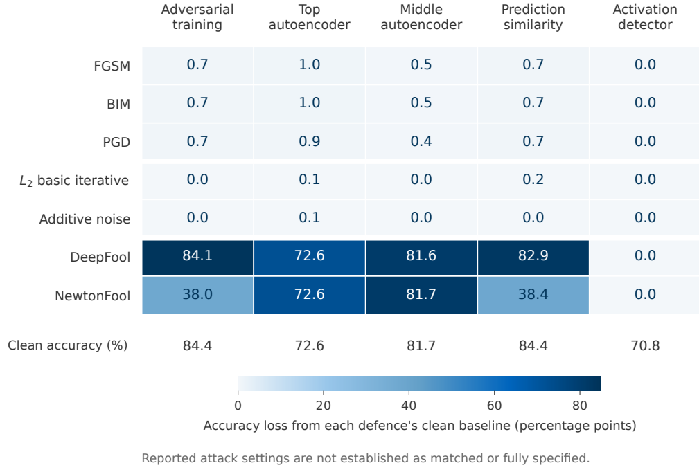
Figure 6.5 Accuracy losses computed from D7.6 Table 2 [39]. Each cell is 100(A_{\text{clean}} - A_{\text{attack}}) in percentage points; the original accuracies remain in Table ?? . The separation of attack rows does not imply matched budgets. In particular, zero loss for the activation detector describes its aggregate score, not a demonstrated mechanism or robustness certificate.
