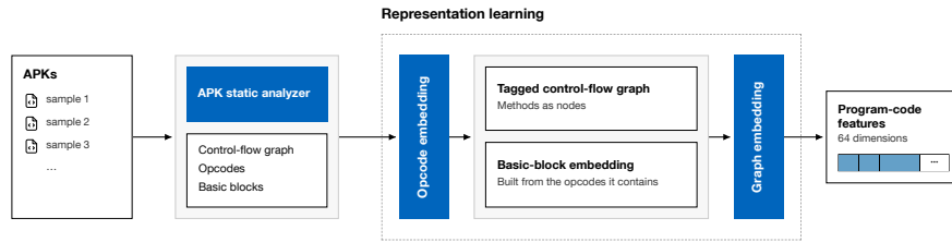
Figure 4.3 The program-code branch. The static analyzer extracts the control-flow graph, opcodes and basic blocks from each APK. Opcodes are embedded first, every method is represented from the tagged control-flow graph of the basic blocks it contains, and a graph embedding reduces the resulting function-call graph to a single 64-dimensional feature vector. Redrawn by the candidate from the arrangement published in [35].
