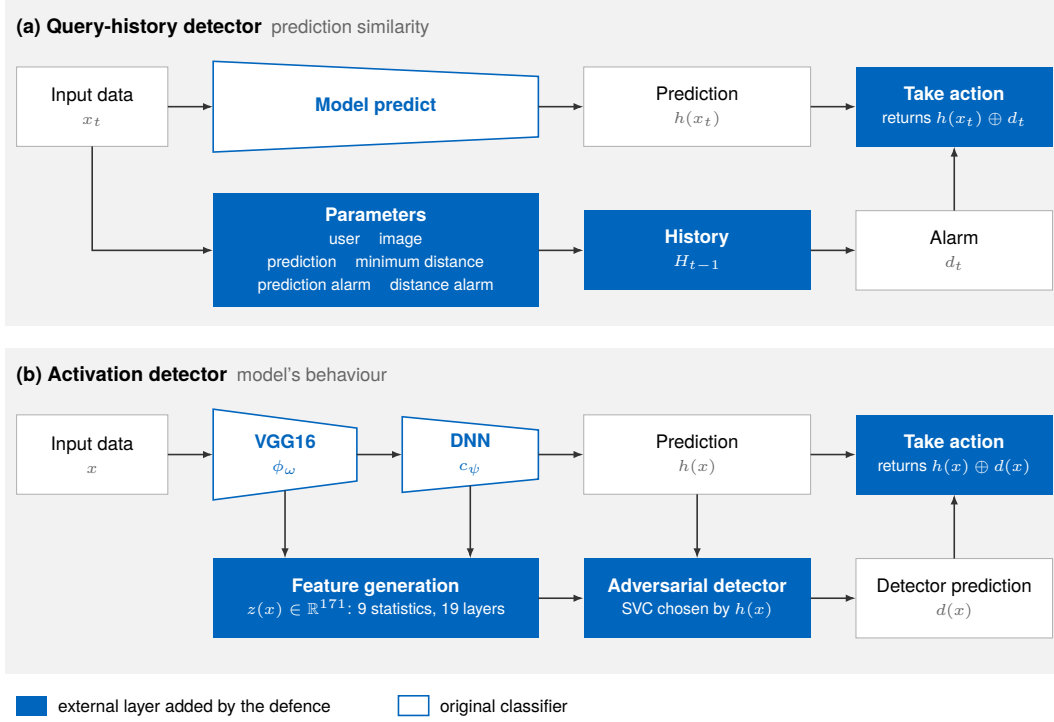
Figure 6.3 Partner detection mechanisms, redrawn after D7.2 Figures 15 and 16, p. 16 [164]. Panel (a) uses preceding queries, whereas panel (b) uses internal activations of the classifier. The recorded parameters, the activation features of Equation ?? and the per-class detector follow D7.2. The response is the label reversal of Equation ??, which D7.6 applies in the benchmark [39]. The final action is part of the defended system and must be included when task accuracy is measured.
