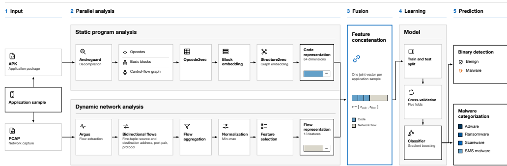
Figure 4.1 The Hybroid architecture. Every application sample provides a pair of inputs: the application package and a capture of the traffic it generates (1). Both are analysed in parallel (2). Androguard decompiles the package into opcodes, basic blocks and a control-flow graph, which are embedded into a 64-dimensional code representation, while Argus turns the capture into bidirectional flows that are aggregated, normalised and reduced to 13 network-flow features. The two representations are concatenated into one joint vector per sample (3), on which a gradient-boosting classifier is trained and cross-validated (4) for binary detection and for categorisation into four malware categories (5). Redrawn by the candidate from the architecture published in [35].
