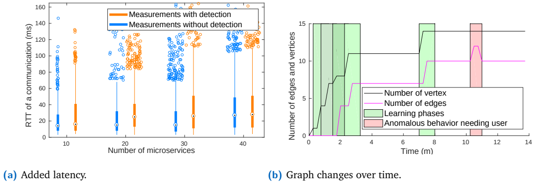
Figure 3.1 The two measurements reported for the service-graph design. Panel (a) gives the inter-service round-trip time with and without detection for ten to forty services. Panel (b) gives the vertex and edge counts of one node's graph over a single run, with the learning phases and the interval of anomalous behaviour shaded. Reproduced from [32], to whose measurement design the candidate contributed.
