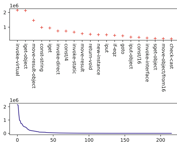
Figure 4.2 Opcode frequency across the pre-training corpus. The upper panel names the twenty most common operations, and the lower panel plots all 216 in rank order, where the shape of the decay is the property the embedding relies on. Reproduced from the candidate’s own publication [35], as is Figure ??.
