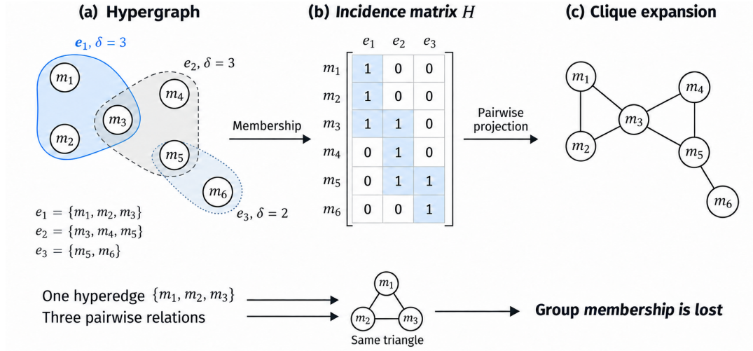
Figure 2.2 The same six methods represented as (a) a hypergraph, (b) its incidence matrix H , and (c) its unweighted clique expansion. A matrix entry is one precisely when the method belongs to the corresponding hyperedge. Hyperedge e_3 joins two vertices and is therefore an ordinary graph edge. The lower example shows that the triangle over m_1, m_2, m_3 arises both from the single hyperedge e_1 and from three separate pairwise relations. The projection preserves pairwise adjacency but does not uniquely determine the original hyperedge memberships [26].
