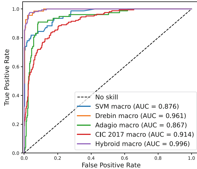
Figure 4.6 Receiver operating characteristic curves for binary malware detection, reproduced from the published vector content of Figure 7 in [35]. The source labels the curves as macro averages and reports the AUC values in the legend. It provides neither a selected operating threshold nor fold-level variation.
