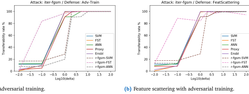
Figure 6.6 Original iterative-FGSM transfer curves from the partner PDF-malware study, D7.5 Figure 15, p. 23 [38]. Both panels retain the published legends and values. The horizontal axis is the source’s \log_{10}(\delta) perturbation budget, distinct from the accuracy loss \Delta used in this chapter. These are feature-space results, with no uncertainty bands or demonstrated construction of modified PDFs with preserved malicious functionality.
