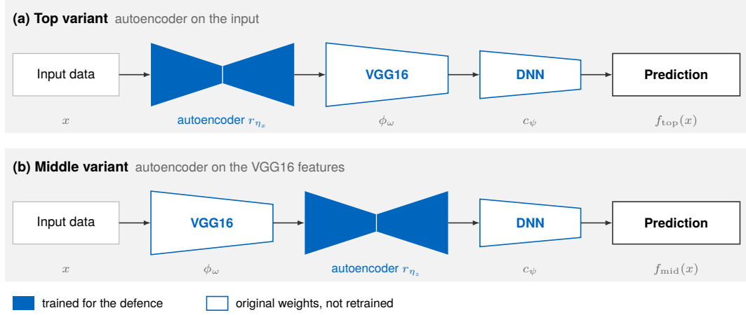
Figure 6.2 Autoencoder placement in the partner classifier, redrawn after D7.2 Figures 13 and 11, p. 14 [164]. In the top variant (a), the autoencoder r_{\eta_x} transforms the input before feature extraction. In the middle variant (b), r_{\eta_z} acts between the feature extractor \phi_\omega and the prediction head c_\psi , as in Equation ?? . The legend follows D7.2, which keeps the original weights of VGG16 and the dense network in both variants. The diagrams specify placement, not a matched ablation of all training choices.
