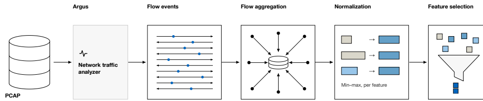
Figure 4.4 The network branch. Argus reduces a raw capture to bidirectional flow events, the events belonging to one application are aggregated into a single record, every attribute is normalised to a common range, and feature selection retains the 13 most informative features. Redrawn by the candidate from the arrangement published in [35].
