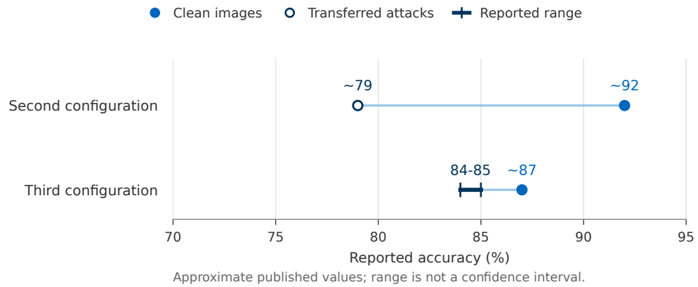
Figure 6.4 SD development configurations from D7.6 Sections 2.8.1.2–2.8.1.3, pp. 18–19 [39]. The interval 84–85% is a reported approximate range, not a confidence interval. The source describes attribute outputs despite its re-identification heading. These values are not additional official contest rows.
