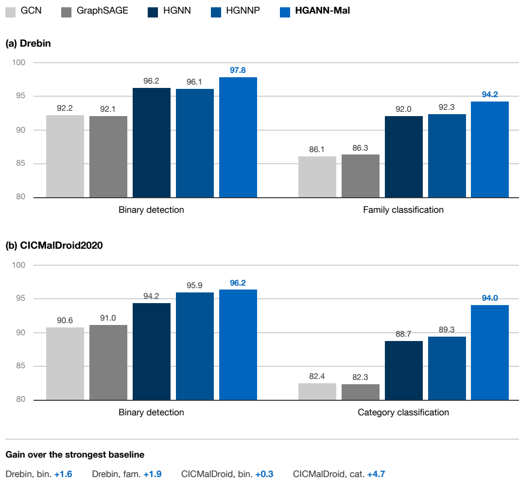
Figure 5.4 F1 on both corpora and both tasks, as published in Tables ?? and ?. The source labels these values Macro-F1, and Section ?? shows that several rows cannot follow one averaging convention. The vertical axis is truncated at 80 so that differences among the hypergraph methods remain visible. HGNNP is the source publication’s name for HGNN+.
