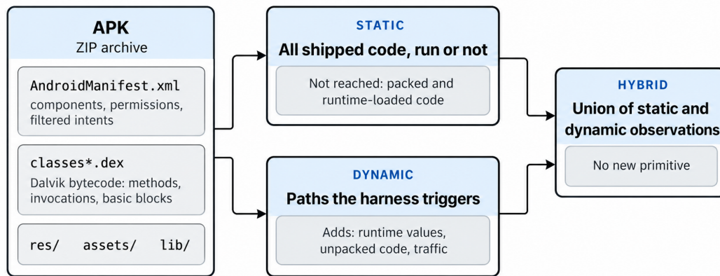
Figure 2.1 What an application package holds and what each mode of analysis reaches. Static observation covers all shipped code and not what the code does; dynamic observation covers what the code did, but only along the paths the harness triggered, and it alone reaches network traffic, which is the channel Chapter ?? uses. The graph objects built from the bytecode are named in Section ??.
