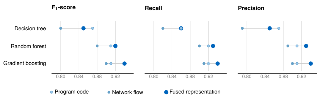
Figure 4.8 Five-class malware-category classification by learner and observation modality, drawn on the same plan as Figure ?? . The score axis is truncated to 0.78–0.96, because this task occupies a lower interval. The values are the five-fold means printed to two decimal places in Figure 9 of [35], checked against the bar geometry of that figure. Decision-tree recall is 0.86 for program code and for the fused representation, so those two markers are drawn concentrically. No fold-level scores are published, so the figure carries no error bars. Redrawn by the candidate.
