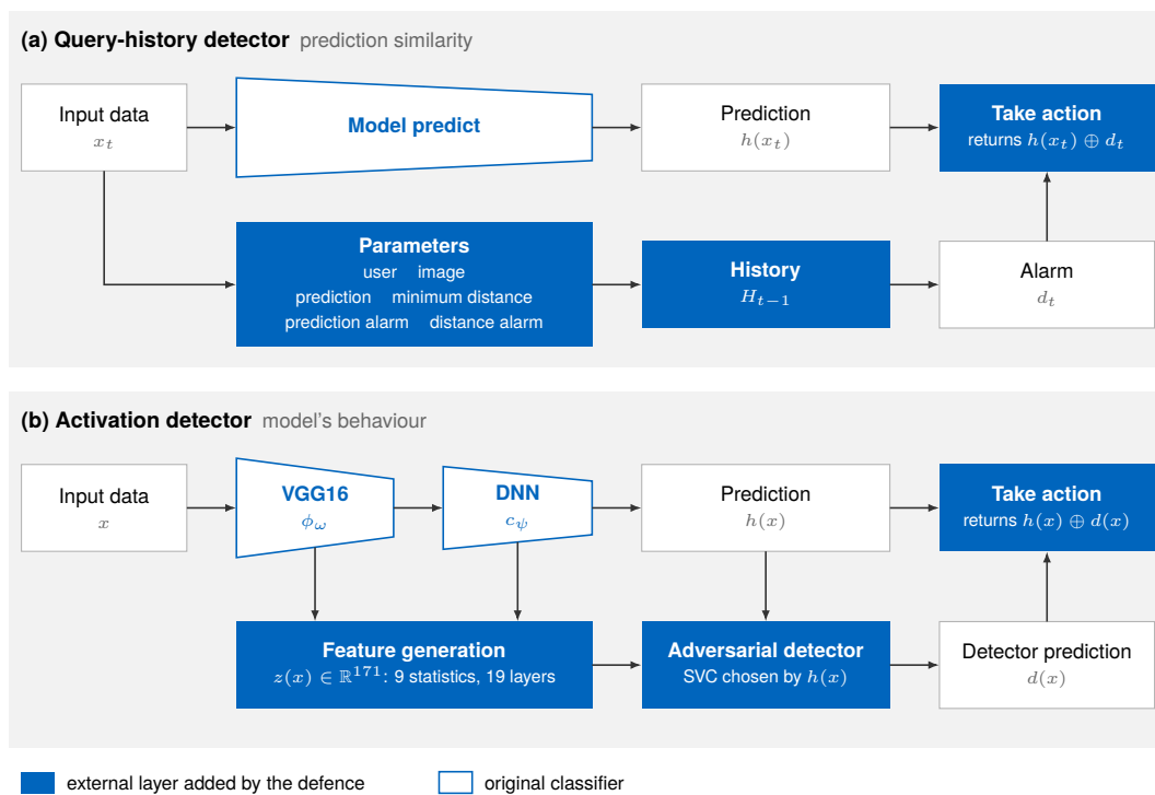
Figure 6.3. Partner detection mechanisms, redrawn after D7.2 Figures 15 and 16, p. 16 [171]. Panel (a) uses preceding queries, whereas panel (b) uses internal activations of the classifier. The recorded parameters, the activation features of Equation 6.9 and the per-class detector follow D7.2. The response is the label reversal of Equation 6.10, which D7.6 applies in the benchmark [39]. The final action is part of the defended system and must be included when task accuracy is measured.
