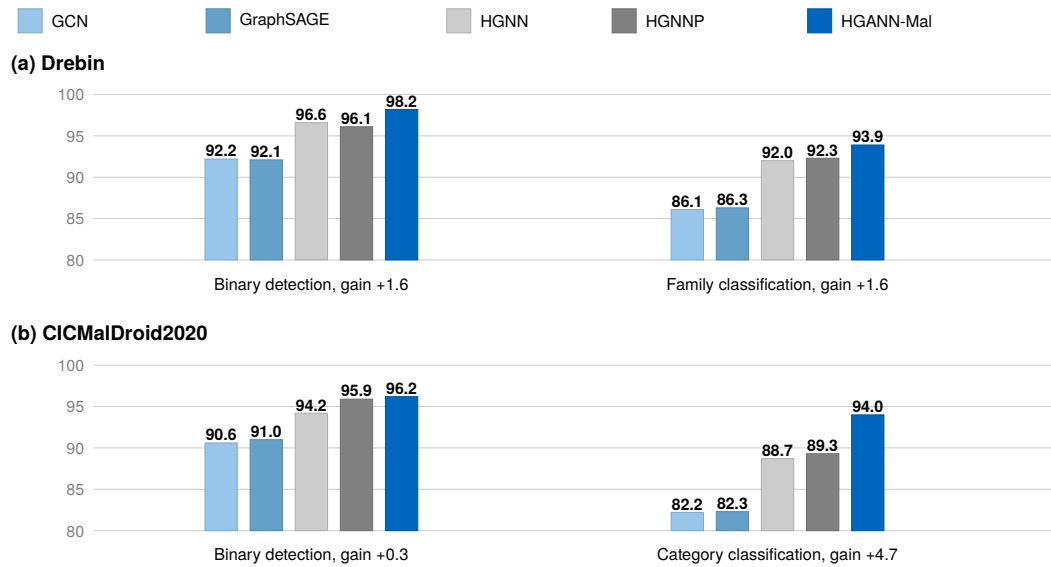
Figure 4.4. Mean Macro- F_1 over five training seeds on each fixed split, from Tables 4.2 and 4.3. The vertical axis is truncated at 80 so that differences among the hypergraph methods remain visible. The gain beside each task is the margin of HGANN-Mal over the strongest baseline. HGNNP is the source publication’s name for HGNN+.
