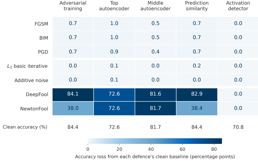
Figure 6.5. Accuracy losses computed from D7.6 Table 2 [39]. Each cell is 100(A_{\text{clean}} - A_{\text{attack}}) in percentage points; the original accuracies remain in Table 6.4. The separation of attack rows does not imply matched budgets. In particular, zero loss for the activation detector describes its aggregate score, not a demonstrated mechanism or robustness certificate.
