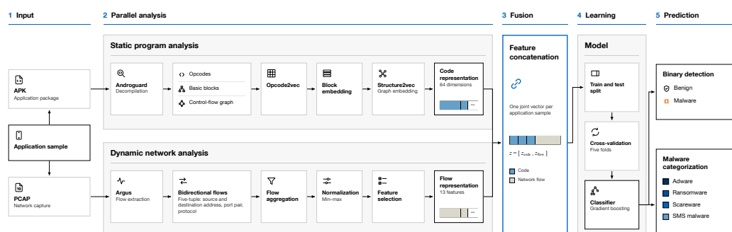
Figure 4.1. The Hybroid architecture, redrawn by the candidate from [35].
