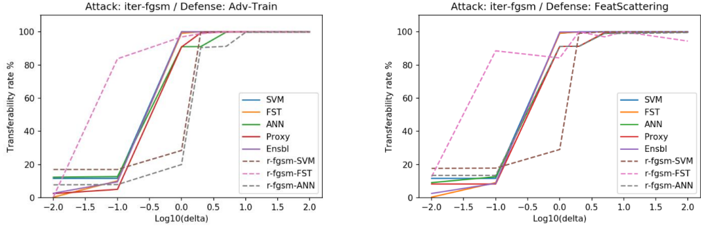
(a) Adversarial training.
