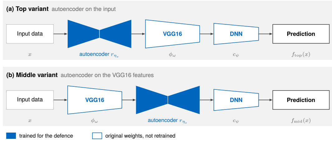
Figure 6.2. Autoencoder placement in the partner classifier, redrawn after D7.2 Figures 13 and 11, p. 14 [173]. In the top variant (a), the autoencoder r_{\eta_x} transforms the input before feature extraction. In the middle variant (b), r_{\eta_z} acts between the feature extractor \phi_\omega and the prediction head c_\psi , as in Equation 6.8.
