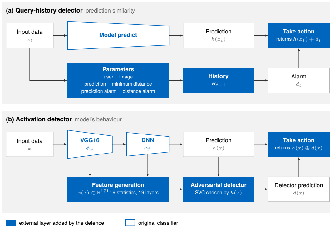
Figure 6.3. Partner detection mechanisms, redrawn after D7.2 Figures 15 and 16, p. 16 [173]. Panel (a) uses preceding queries, whereas panel (b) uses internal activations of the classifier. The recorded parameters, the activation features of Equation 6.9 and the per-class detector follow D7.2. The response is the label reversal of Equation 6.10, which D7.6 applies in the benchmark [39]. The final action is part of the defended system and must be included when task accuracy is measured.
