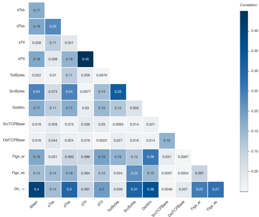
Figure 4.5. Kendall correlation among the retained flow features, used to check that the selected features are not redundant with one another.
