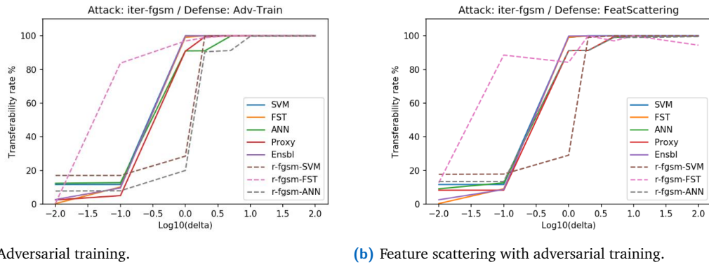
Figure 6.6. Original iterative-FGSM transfer curves from the partner PDF-malware study, D7.5 Figure 15, p. 23 [38]. Both panels retain the published legends and values. The horizontal axis is the source's \log_{10}(\delta) perturbation budget, distinct from the accuracy loss \Delta used in this chapter. These are feature-space results, with no uncertainty bands or demonstrated construction of modified PDFs with preserved malicious functionality.
