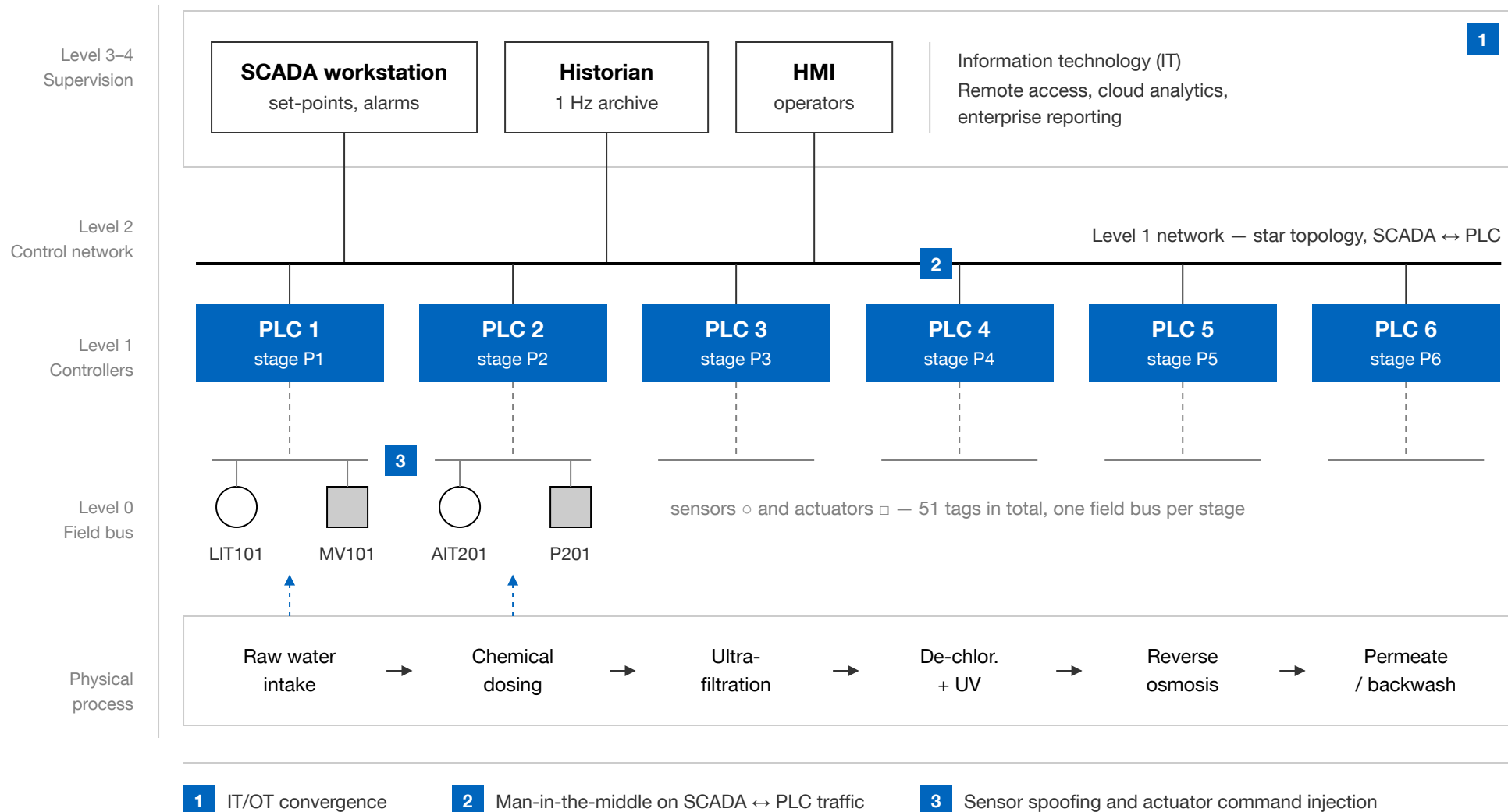
Figure 2.1: Layered architecture of an industrial control system. Six programmable logic controllers, each responsible for one process stage, exchange set-points and measurements with the SCADA workstation over a Level 1 star network, while a Level 0 field bus connects each controller to its own sensors and actuators. The three numbered positions are the attack surfaces exposed by the convergence of information and operational technology.
