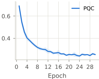
(b) Training loss
