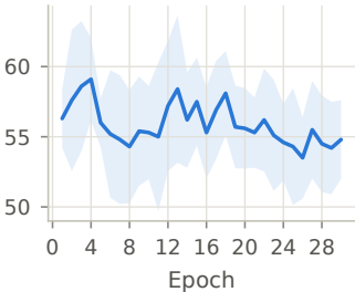
(a) Validation accuracy (%)
