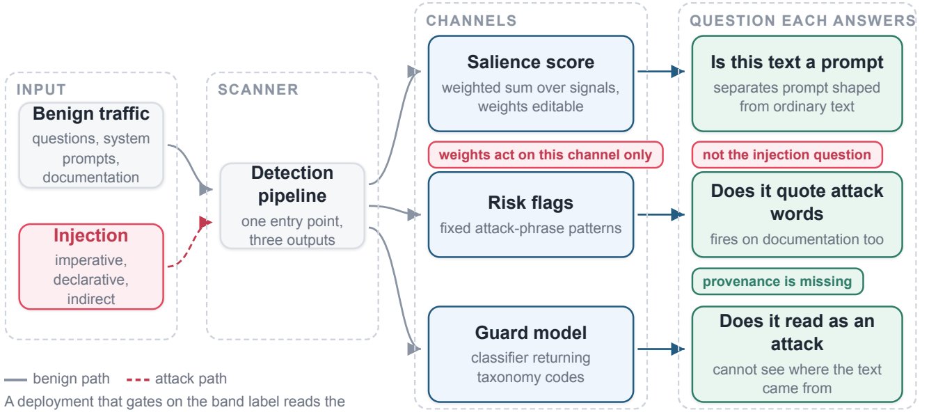
Fig. 1: The three outputs of the detector and the question each one decides, established in Sections VII and X. The weighted score is recovered by a code-aware detector and reports whether text is prompt shaped. The flag channel matches attack vocabulary. The guard model reads the text. None of the three receives the provenance of the text, which is what separates an authorised instruction from an injected one, and which provenance-marking defences supply at the architecture level [2], [16], [17].
