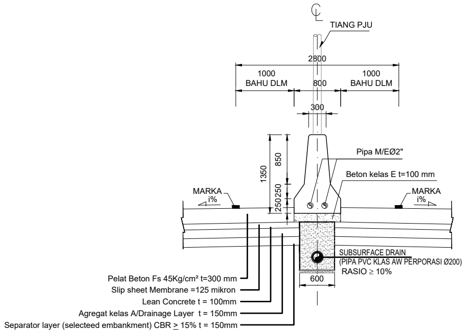
DETAIL D MEDIAN AKSES KONDISI NORMAL
