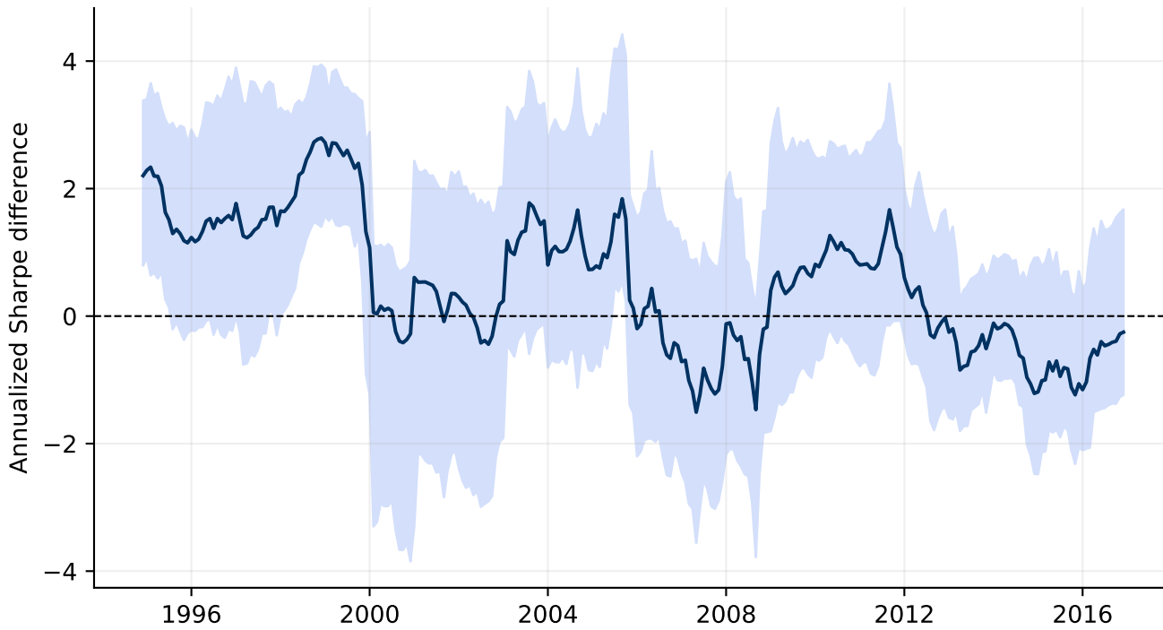
Extension LSTM minus Transformer 36-month windows
