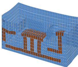
(c) robust design: part sectioned at y = 0 (mean copper density 0.927)
