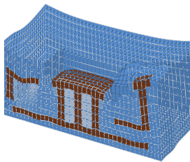
(a) baseline: part sectioned at y = 0 (mean copper density 0.959)
