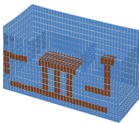
(b) nominal optimum: part sectioned at y = 0 (mean copper density 0.929)
