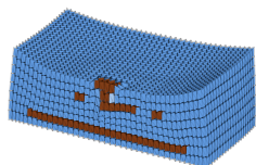
(a) baseline: sectioned part
