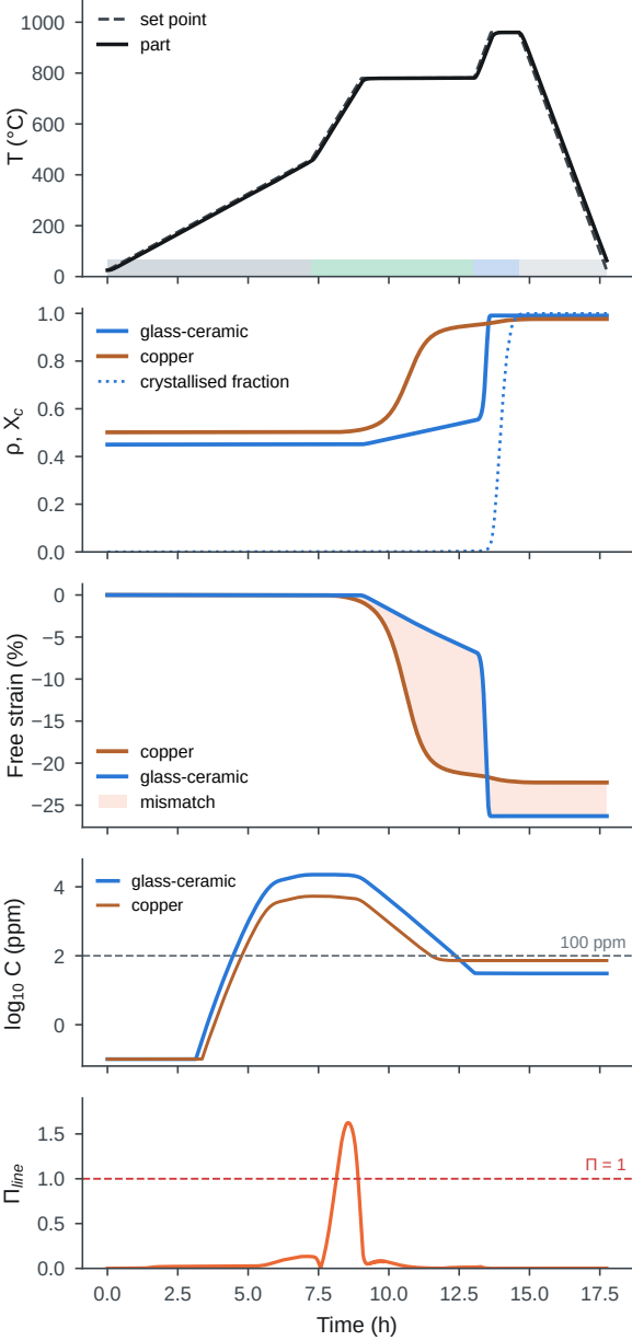
(a) baseline: 3 \mu\text{m} Cu, burnout 780 ^{\circ}\text{C} / 4 h, peak 960 ^{\circ}\text{C}
