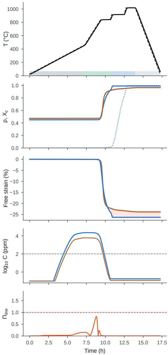
(b) optimised: 3.9 \mu\text{m} Cu + 24 % filler, burnout 840 ^{\circ}\text{C} , holds 916 / 1018 ^{\circ}\text{C}
