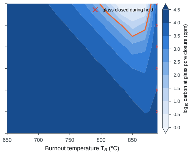
(b) 4 % H_2 through a +20 °C bubbler
