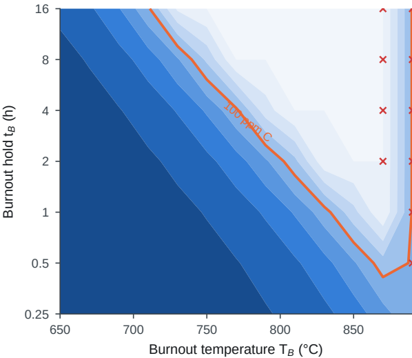
(a) 30 % steam, H_2 at 20 % of Cu/Cu_2O limit
