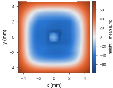
(c) top surface, range 150 \mu\text{m}
