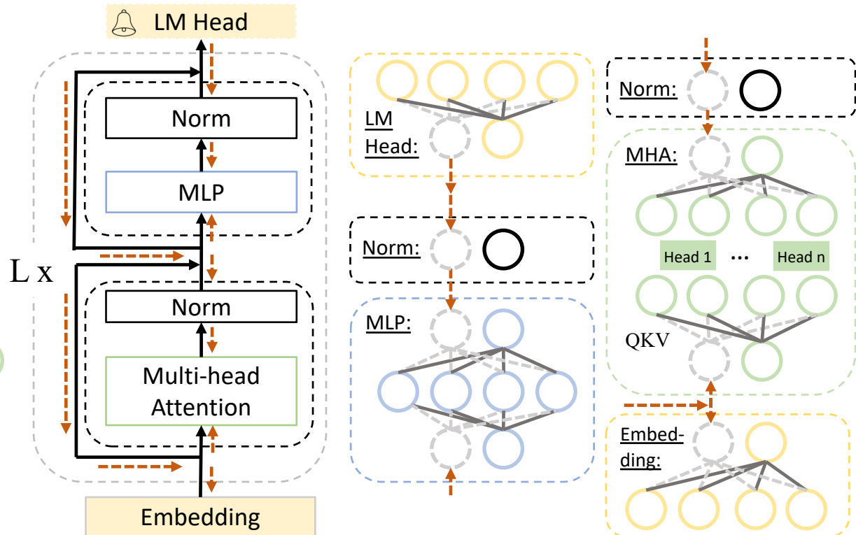
Group Type C: Channel-wise Grouping
