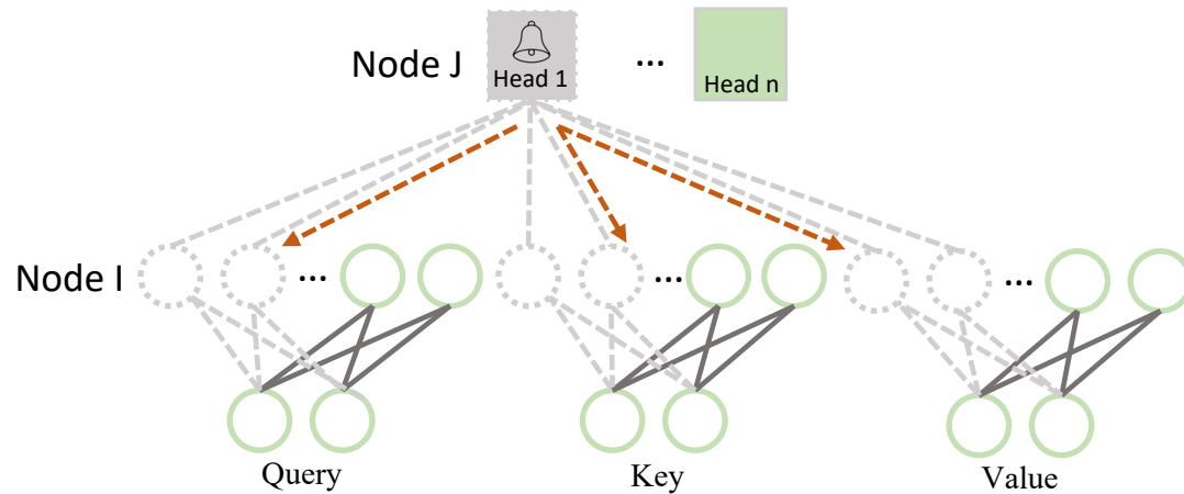
Case 2: Node I is dependent on Node J
