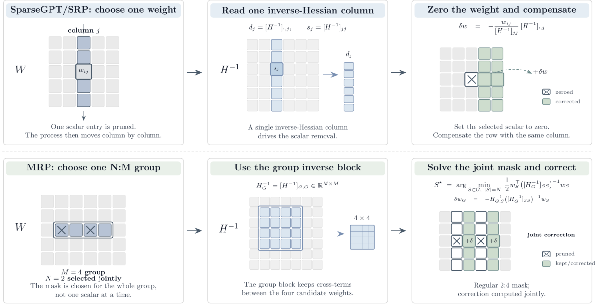
Figure 5.1: Second-order compensation strategies for unstructured and semi-structured pruning. SparseGPT removes one scalar weight per step and compensates using one column of \hat{H}^{-1} , while MRP removes an N:M group jointly and uses the block (\hat{H}_{MM}^{-1})^{-1} to model interactions among simultaneously removed weights.
