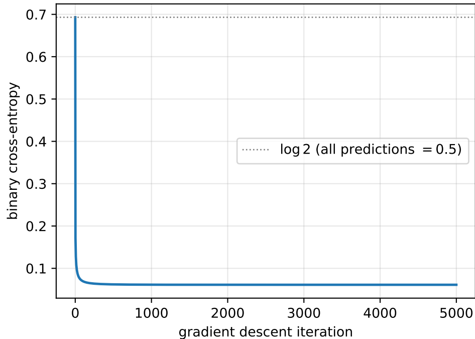
Training loss, \eta = 0.5
