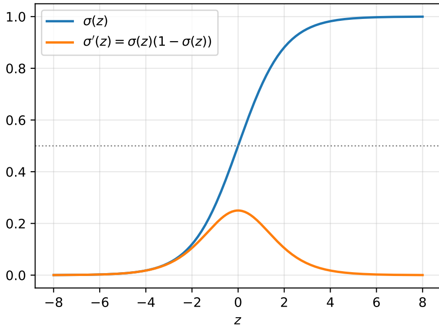
Sigmoid and its derivative
