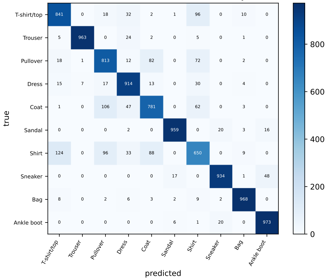
Fashion-MNIST test confusion matrix (accuracy = 0.8796)
