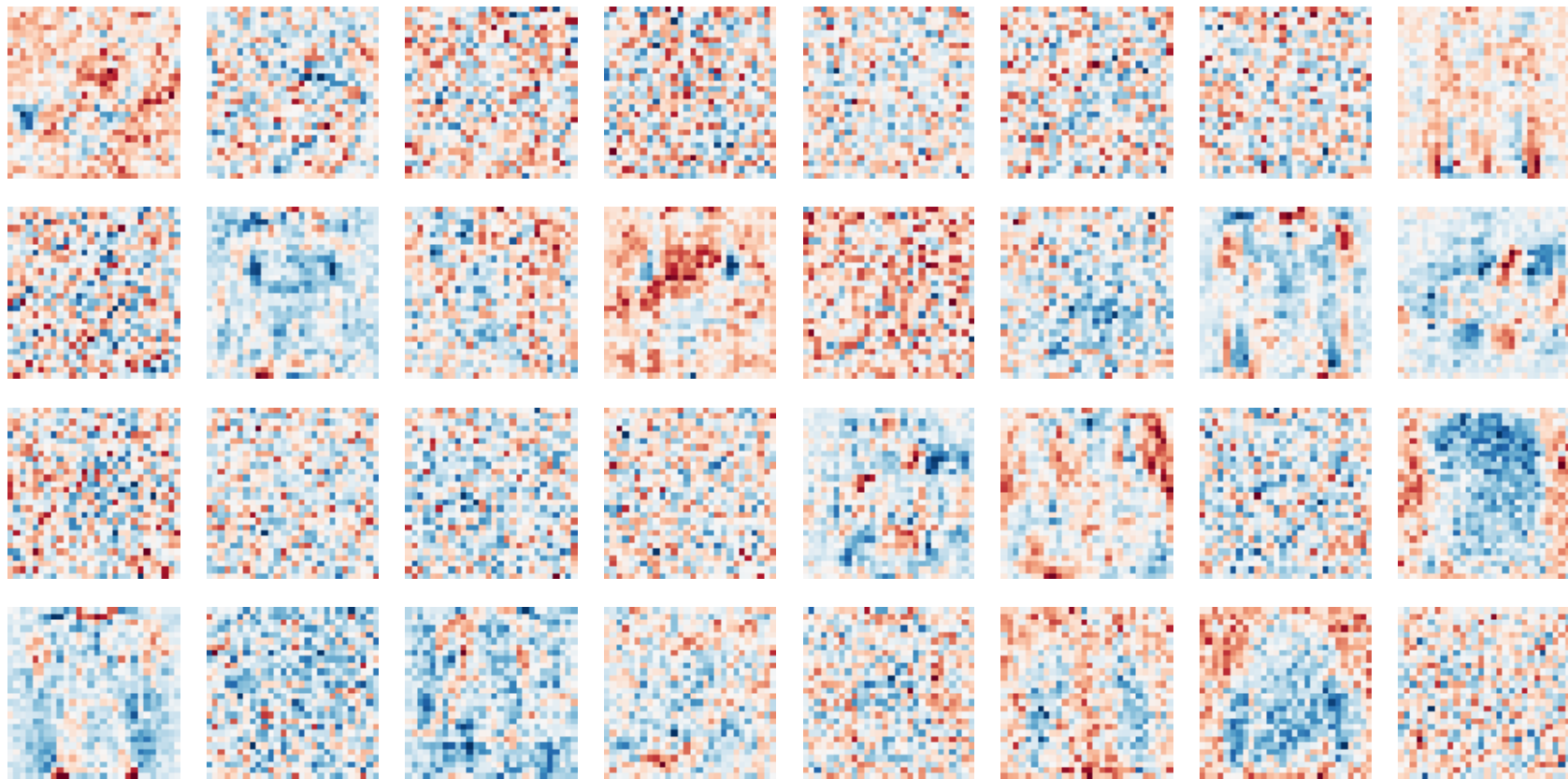
First-layer weights, one column of W_1 per image
