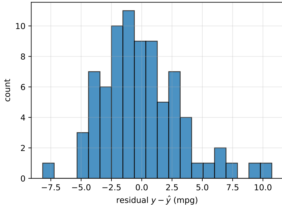
Residual distribution
