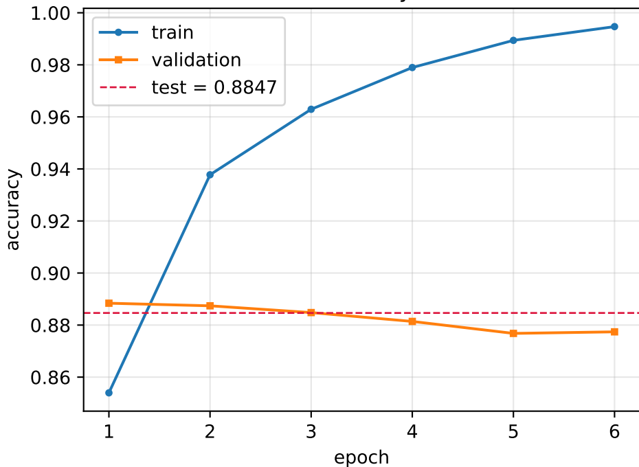
Accuracy
