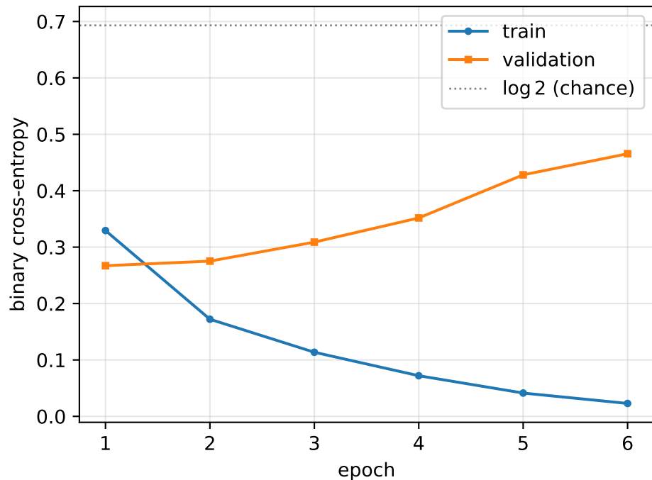
Loss
