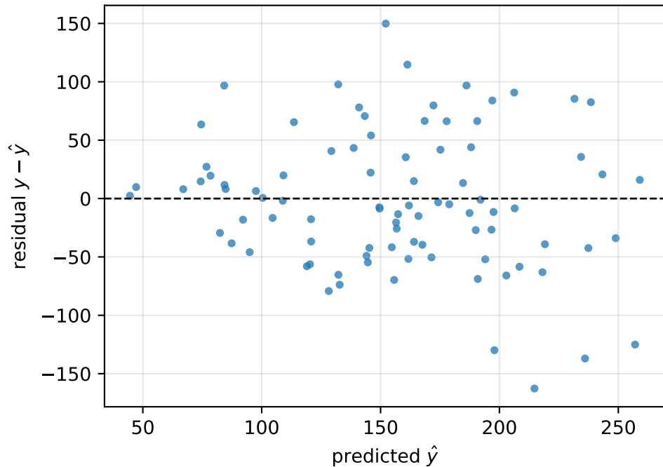
Residuals vs fitted values
