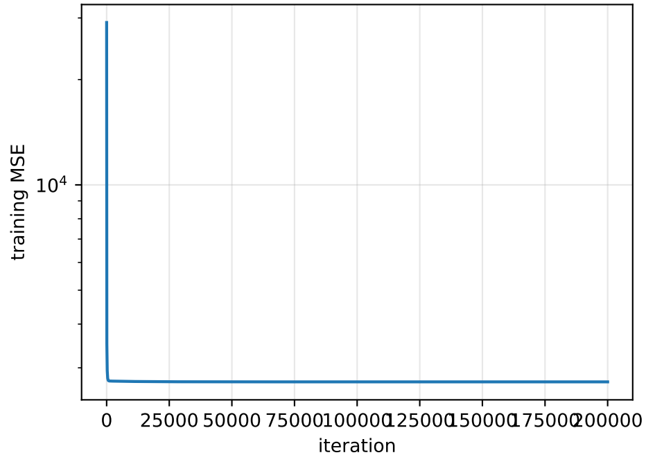
Gradient descent, \eta = 0.9
