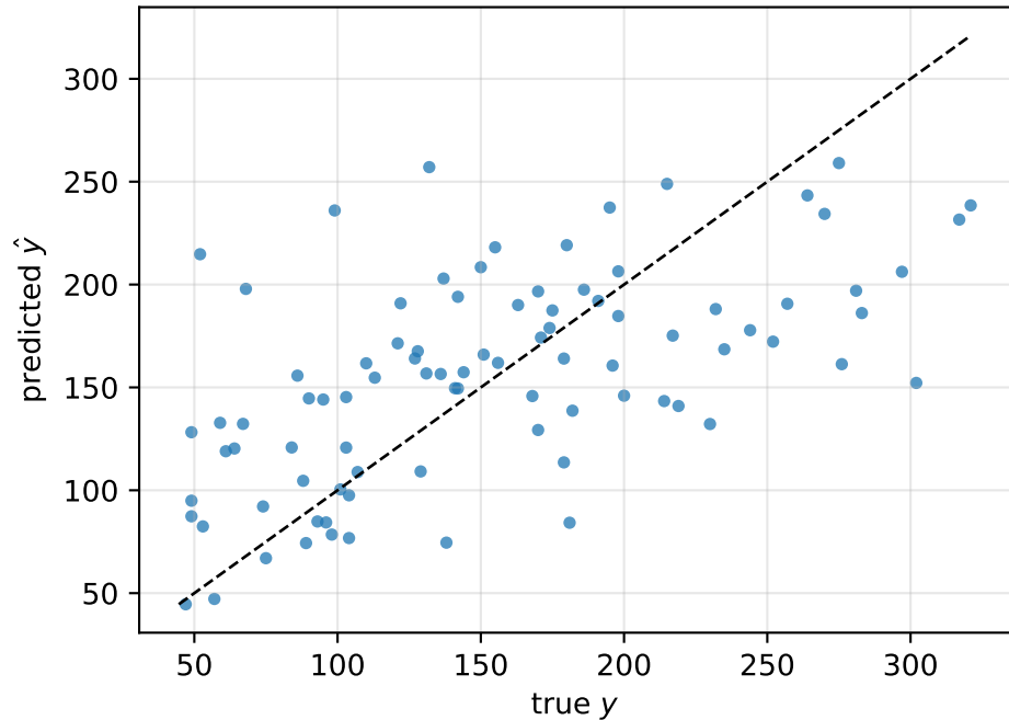
Test set, R^2 = 0.332
