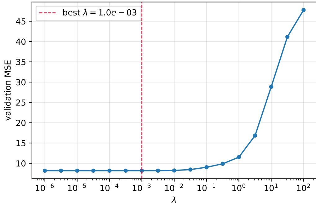
Choosing the penalty strength
