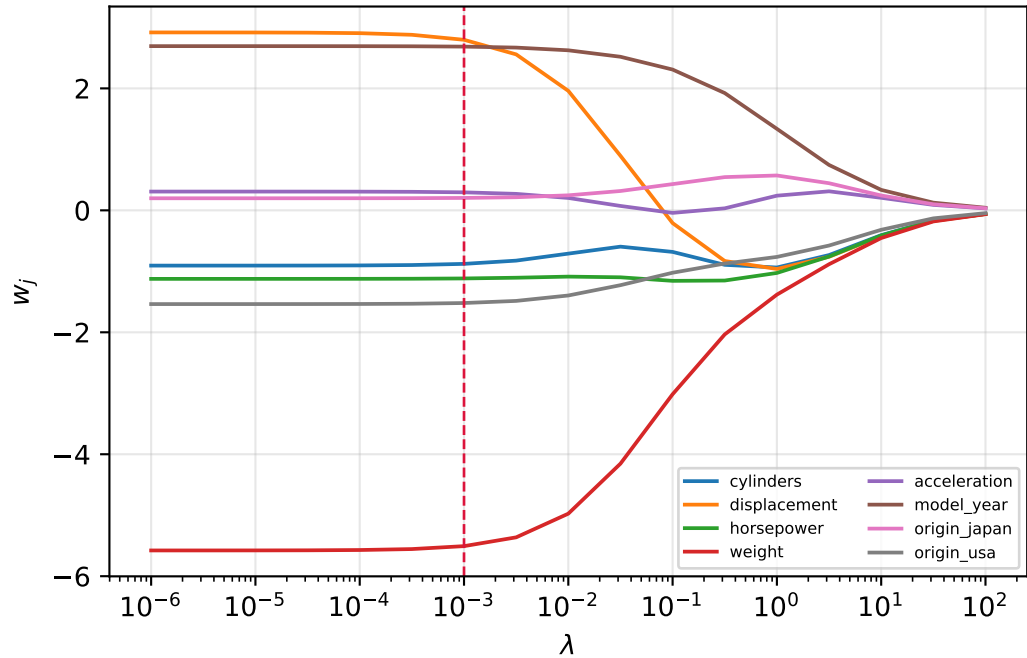
Weights shrink as \lambda grows
