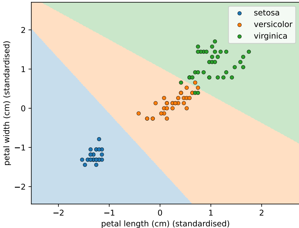
Decision regions (the boundaries are straight lines)
