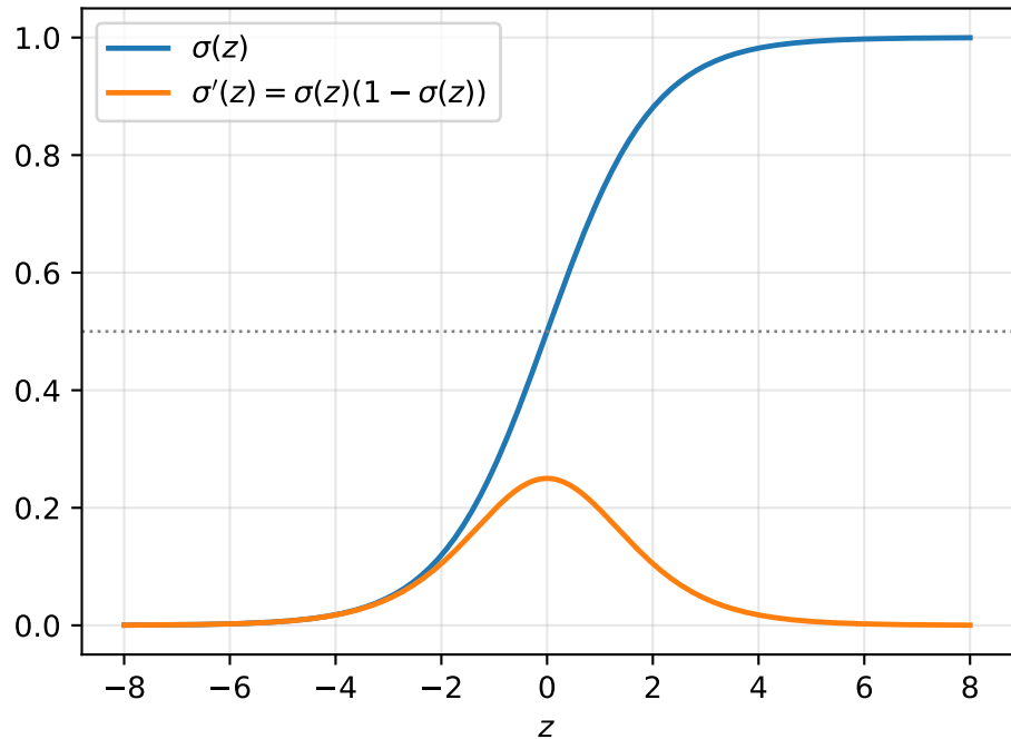
Sigmoid and its derivative
