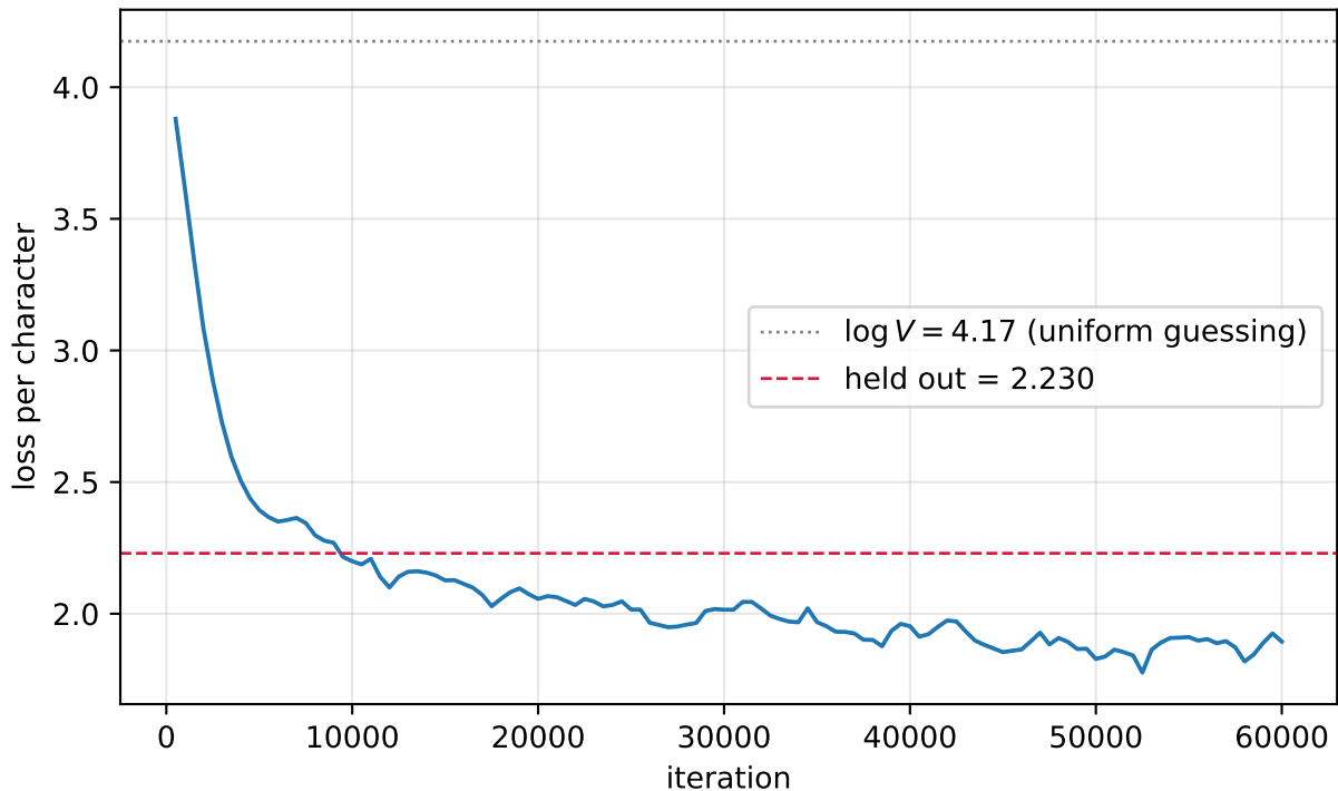
Training a character RNN
