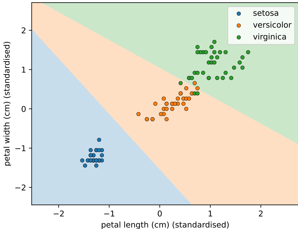
Softmax decision regions (linear boundaries)
