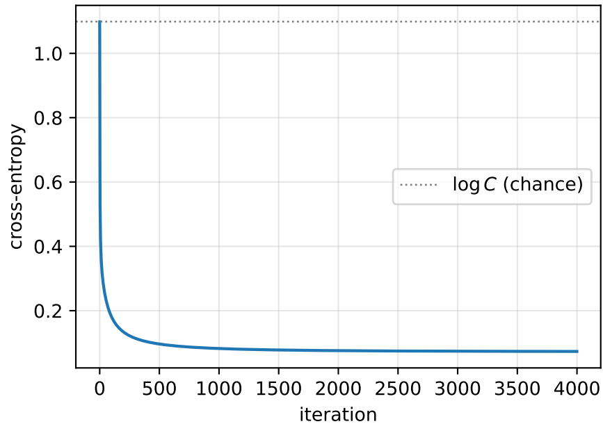
Softmax regression training, \eta = 0.5
