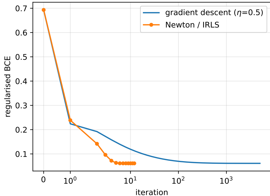
First order vs second order optimisation
