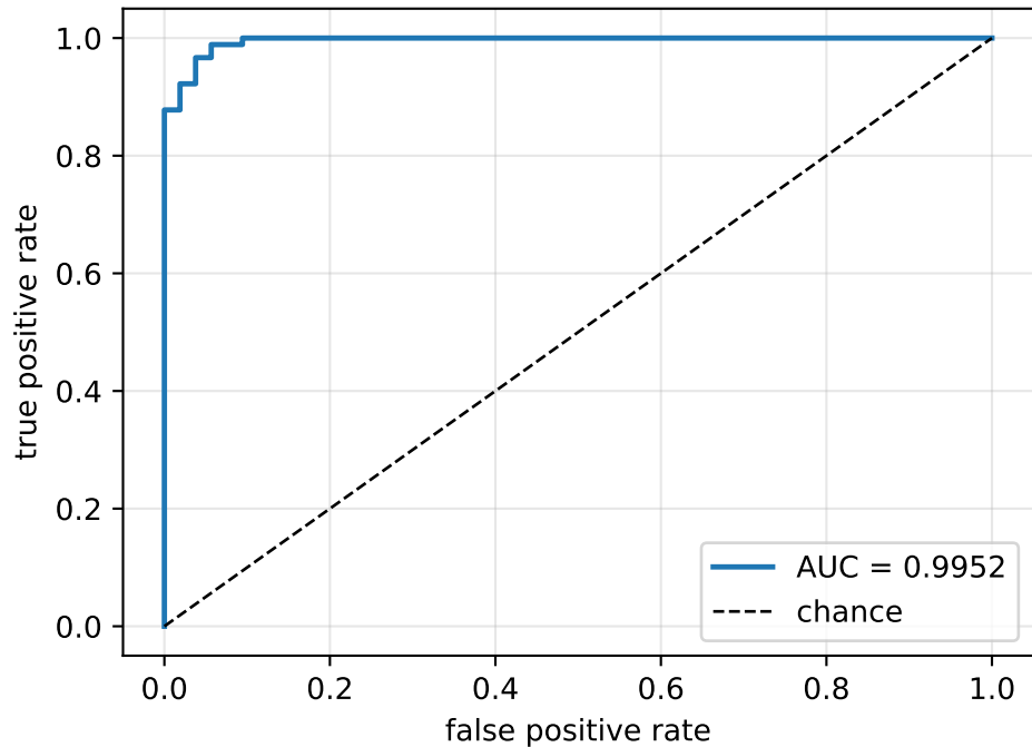
ROC curve (test set)
