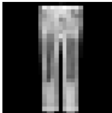
Trouser (Trouser)
