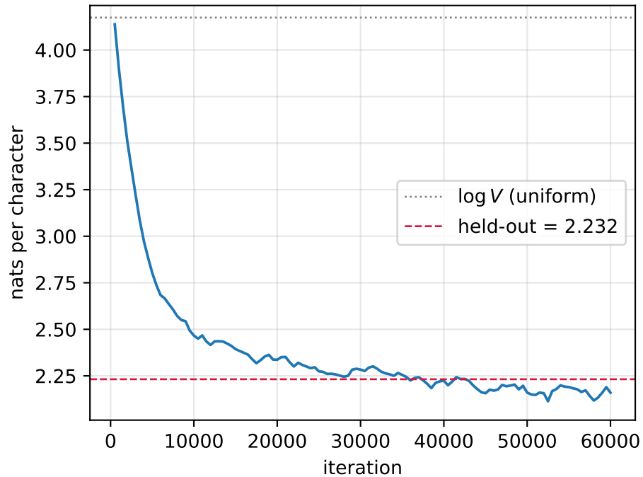
Smoothed training loss (Adagrad + BPTT)
