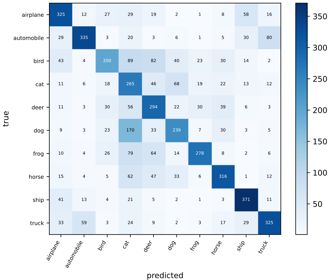
CIFAR-10 test confusion matrix (acc = 0.5896)
