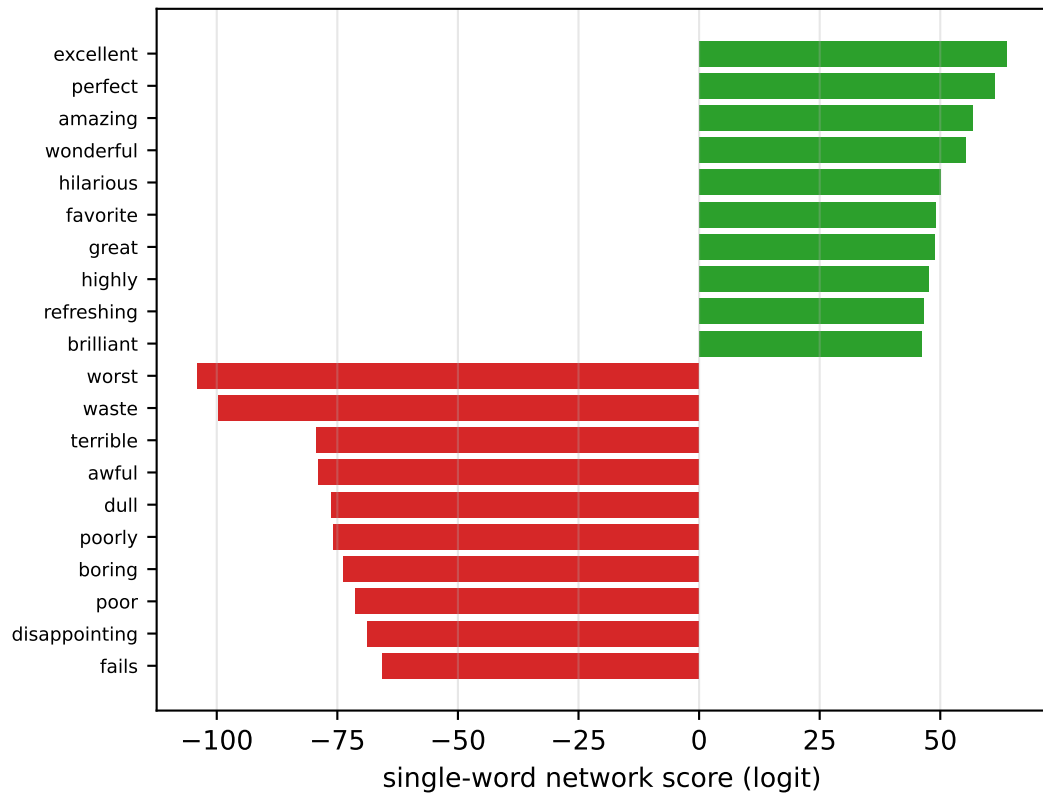
Most polarised vocabulary items
