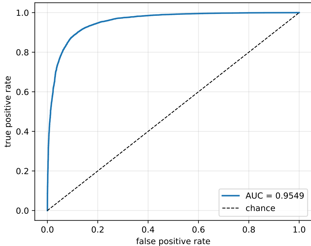
ROC curve (test set)
