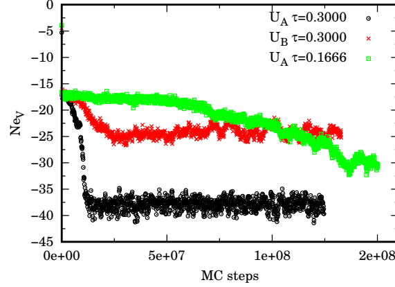
FIG. 9. We show the evolution of the potential energy NeV during the simulation of case E\mathcal{A} ( U_{\mathcal{A}} \tau = 0.3 ) and E\mathcal{B} ( U_{\mathcal{B}} \tau = 0.3 ) and for the same bosonic mixture treated with the inter-action \mathcal{A} with a smaller timestep \tau = 0.1666 for M = 200 . For case E\mathcal{A} with \tau = 0.3 we see an abrupt ‘transition’ at about 10^7 MC steps when the blob shown in Fig. 8 is formed. The energy is in units of a Hartree.
