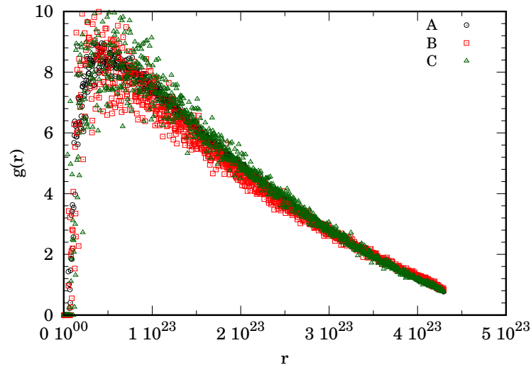
FIG. 1. The RDF for cases A,B,C of Table I. The radial distance r is in Planck units 1.61623 \times 10^{-33} cm. The radial length of the patch is \delta = 4.3 \times 10^{23} .
