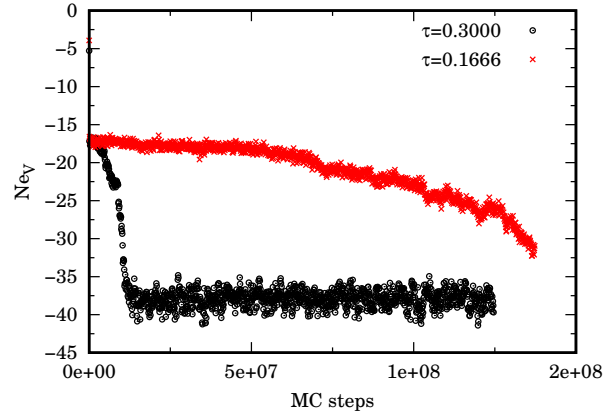
FIG. 9. We show the evolution of the potential energy N_e V during the simulation of case E and G. The energy is in units of a Hartree. For case E we see a ‘transition’ at about 10^7 MC steps when the blob shown in Fig. 6 is formed.
