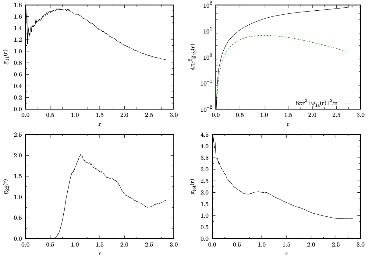
FIG. 7. We show the partial and total RDF of the H fluid for cases G in Table I where \tau = 0.1666 . In the panel for the unlike radial distribution function we also show the ground state probability distribution of the H atom |\psi_{1s}|^2 for comparison. The peak in g_{22} reflects the formation of the \text{H}_2 molecules. The distance r is in units of a Bohr radius.
