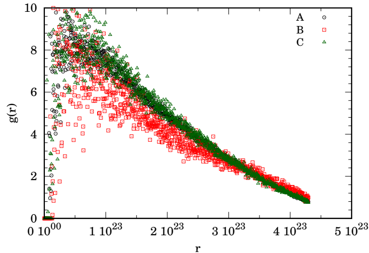
FIG. 1. The RDF for cases A,B,C of Table I. The radial distance r is in Planck units 1.61623 \times 10^{-33} cm. The radial length of the patch is \delta = 4.3 \times 10^{23} in Planck units.
