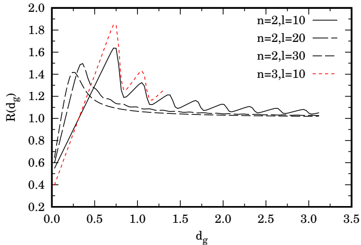
FIG. 1. We show the plot of the ratio R(m\delta) = P(m\delta; n\tau)/n\tau\phi(m\delta) as a function of m\delta for a = 1, \mu_1 = \mu_2 = 1, Z_1 = -Z_2 = -1, \tau = 0.01, \delta = 0.03 and n = 2, l = 30 and n = 3, l = 10 . The oscillations observed for l = 10 are a numerical artifact of the error in the calculation of the angular convolutions. From the case n = 2 we see how already for l = 30 the squaring is close to convergence. But for n = 3 the case l = 30 is prohibitively computationally demanding.
