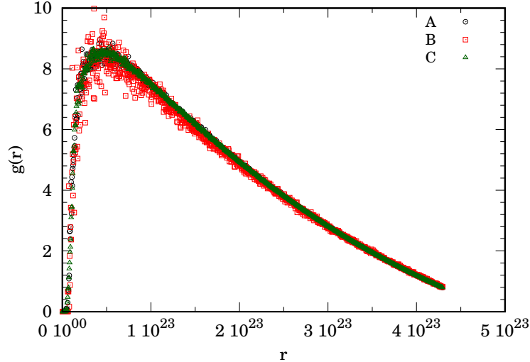
FIG. 1. The RDF for cases A,B,C of Table I without permutations. The radial distance r is in Planck units 1.61623 \times 10^{-33}\text{cm} . The radial length of the patch is \delta = 4.3 \times 10^{23} .
