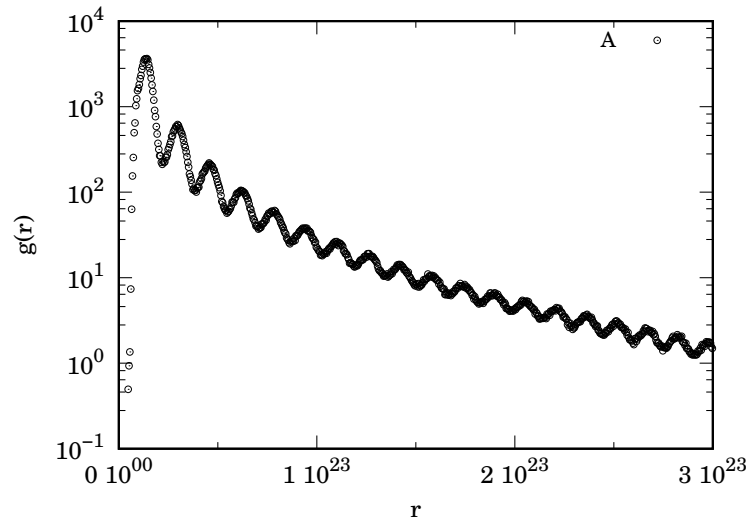
FIG. 1. The RDF for case A of Table I. The radial distance r is in Planck units 1.61623 \times 10^{-33} cm. A logarithmic scale is used on the y -axis.
