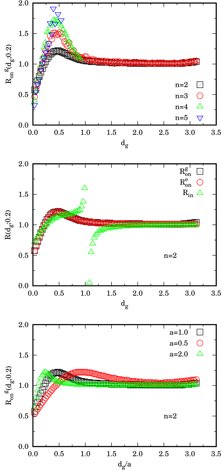
FIG. 1. We show the plot of the ratio R(d_g; t) = P(m\delta; t)/t\phi(m\delta) as a function of d_g = m\delta for a = 1, \mu_1 = \mu_2 = 1, Z_1 = Z_2 = 1, t = n\tau = 0.2, \delta = 0.03 . On the top panel R_{\text{on}}^g for n = 2, 3, 4, 5 . On the central panel the three Coulomb cases R_{\text{on}}^g, R_{\text{on}}^e, R_{\text{in}} for n = 2 . On the bottom panel the case R_{\text{on}}^g for n = 2 and different Sphere radii. The angular convolutions in Eq. (2.11) were calculated with a Monte Carlo quadrature with no less than 10^6 MC points and keeping the relative statistical error below 10% for n < 5 and below 40% for n \geq 5 (this required approximately > 5 \times 10^8 MC points in the n > 5 case).
